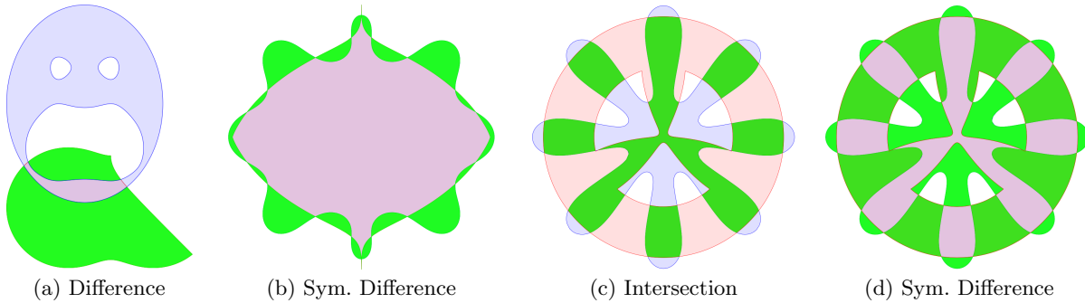
Figure 2: Boolean set operations on algebraic polygons (red and blue) each defined by a bounded face of a curve’s arrangement. Degree of curves: (a) blue: 10, red: 7 (b) blue: 16, red: 14, (c+d) blue: 16, red: union of two degree 4 curves
