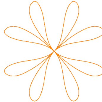
Figure 4: A curve of degree 16 with a highly degenerate singularity. Our software computes the arrangement induced by the curve correctly, i.e., returns an arrangement with 9 faces and a vertex with 16 incident edges.
