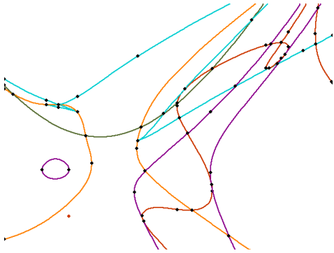
Figure 5: Arrangement of curves needed to analyse and decompose two random surfaces of degree 3 and 4 following the approach in [16] (cutout). Singular points and tangential intersections naturally appear in this task. The full arrangement consists of 111 vertices (3 of which are isolated), 164 edges and 61 faces.
