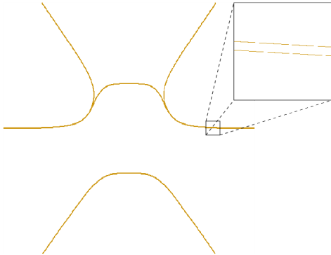
Figure 3: The curve with equation y^{10} - 2(x^4 y - 1)^2 . Note that for any x > 1 , the fiber consists of the roots of a Mignotte polynomial of type x^n - 2(ax - 1)^2 which is known to have a bad root separation [36]. Consequently, two arcs of the curve have extremely small distance from each other. Our software computes the arrangement induced by this curve almost instantly (about 1 second), correctly separating these arcs.
